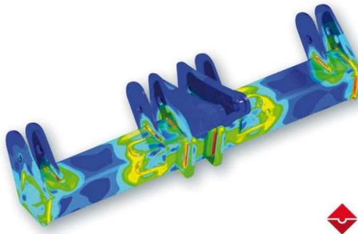
Simufact-GR-Simufact.welding-Simulation-carrier-residual-stress
