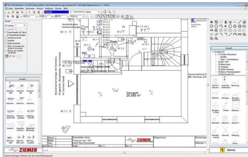
SCC-CAD Startup
