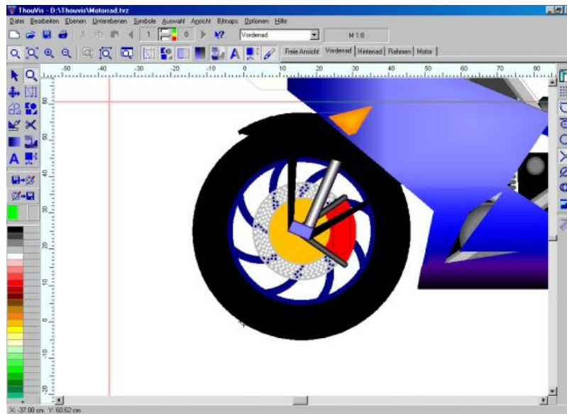
Screenshot ThouVis 1.0
