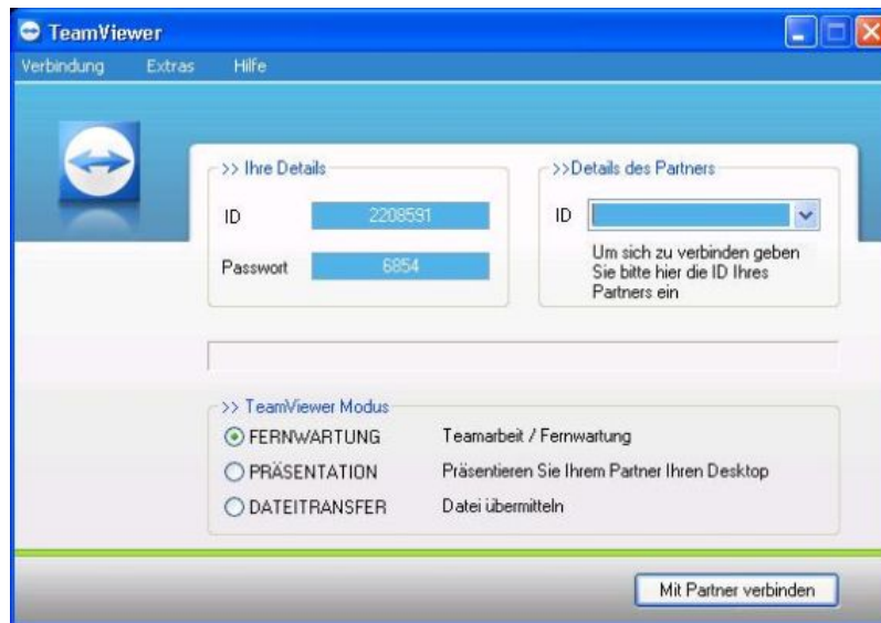
TeamViewer
